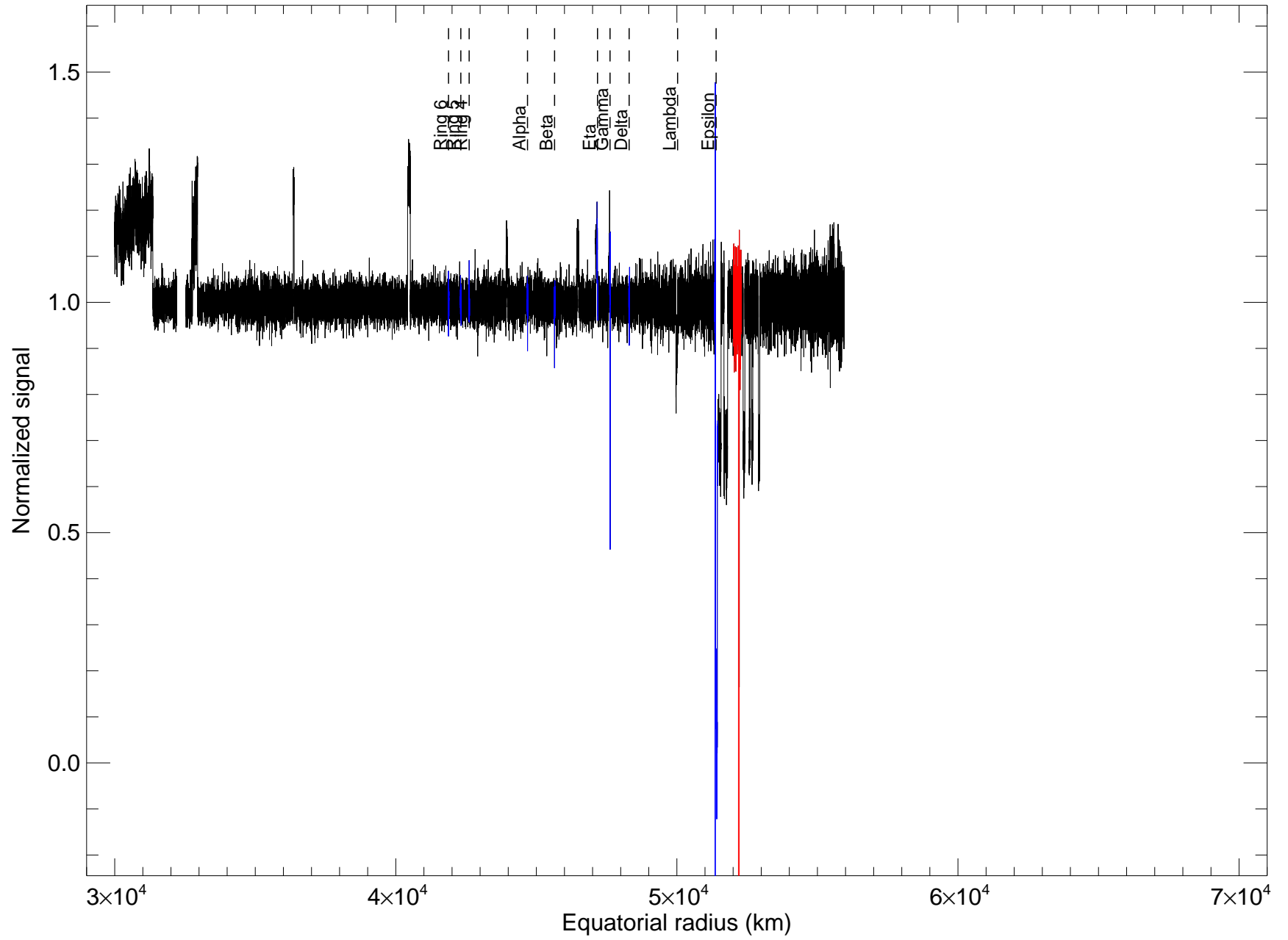
u34_irtf_320cm_2200nm rings egress
