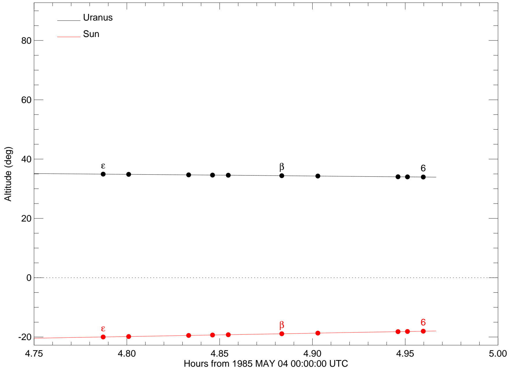
u23 observed from Observatorio del Teide 155cm
