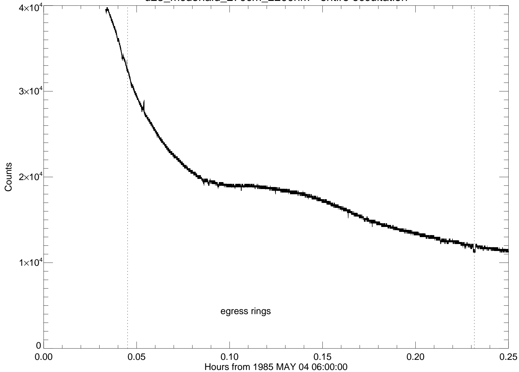
u23_mcdonald_270cm_2200nm - entire occultation
