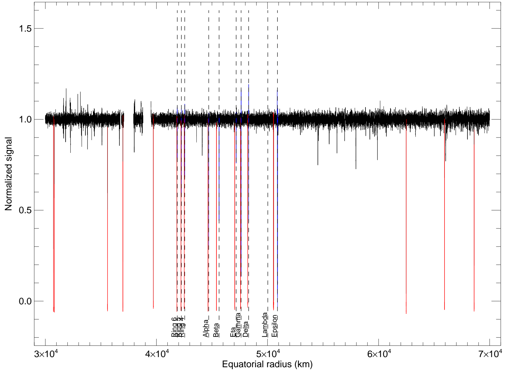
u17b_saao_188cm_2220nm rings ingress
