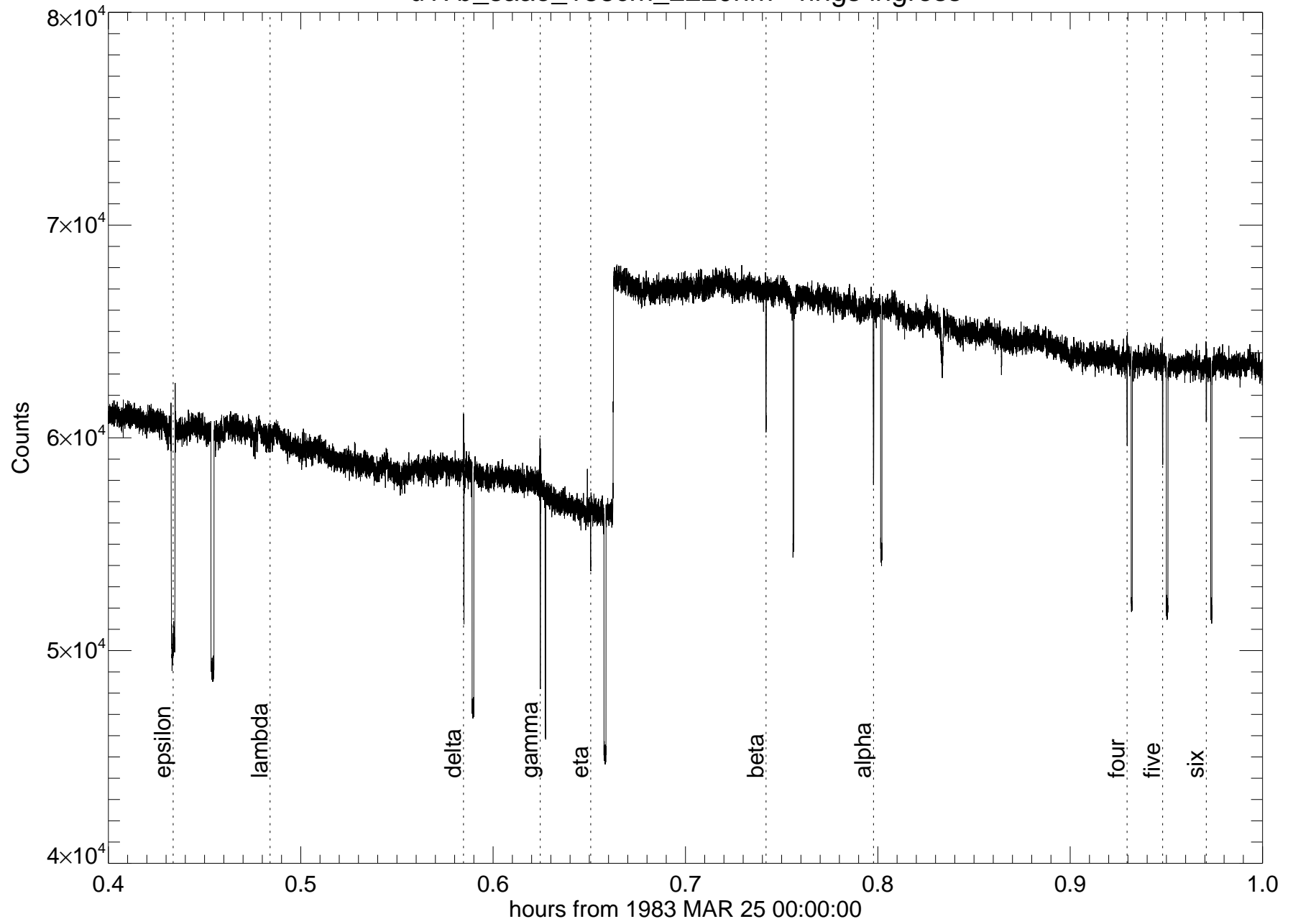
u17b_saao_188cm_2220nm - rings ingress
