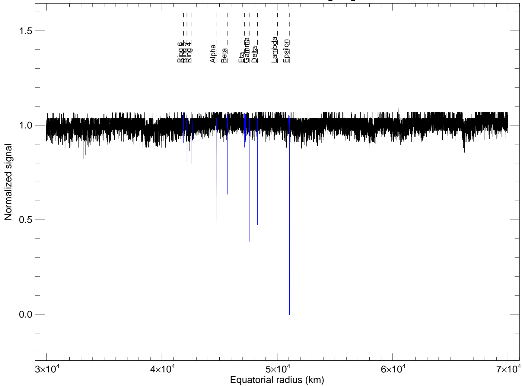
u14_ico_250cm_2200nm rings egress
