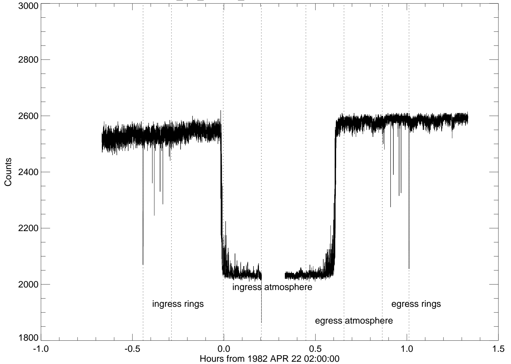
u14_lco_250cm_2200nm - entire occultation
