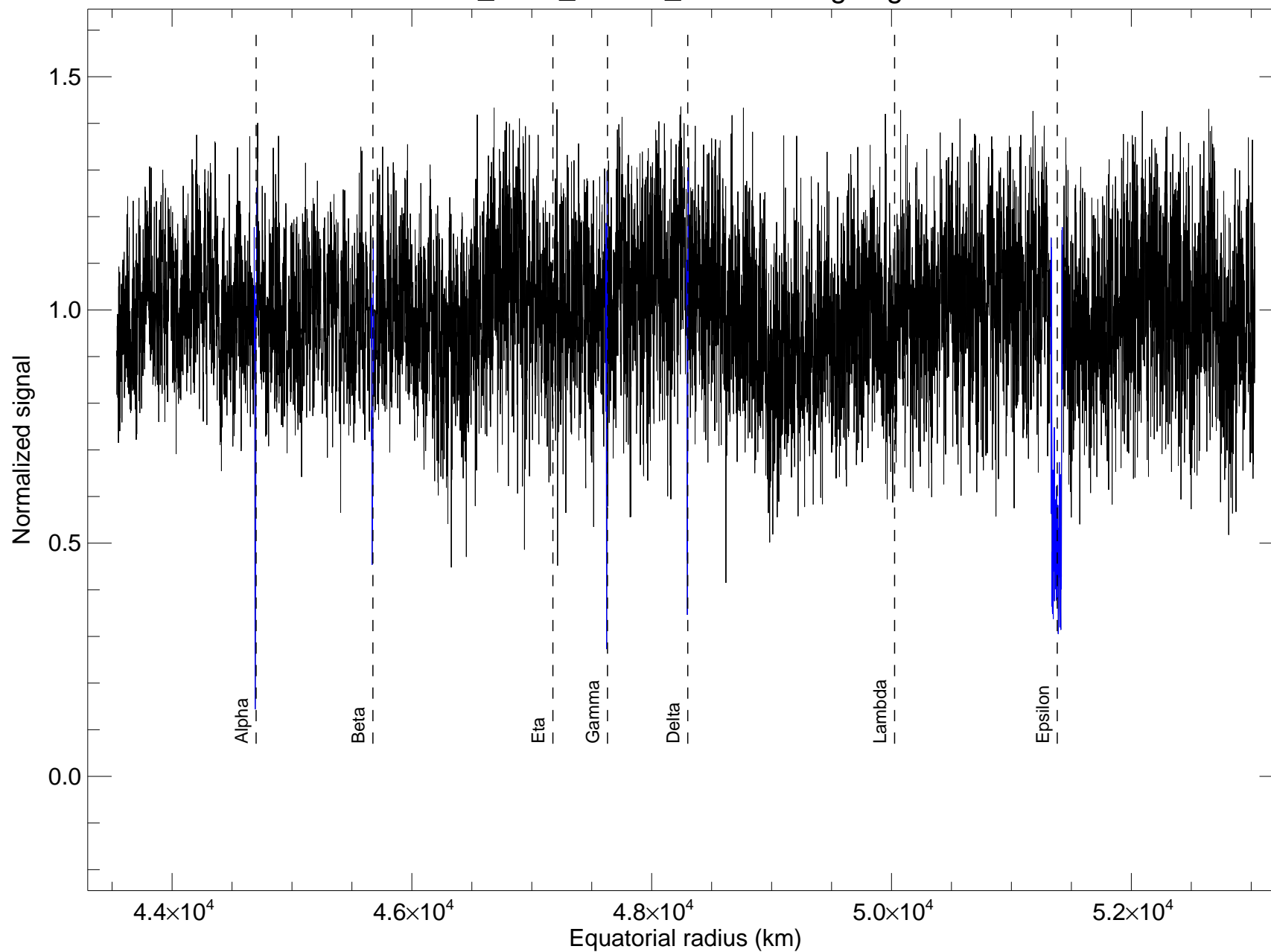
u144_caha_123cm_2200nm rings egress
