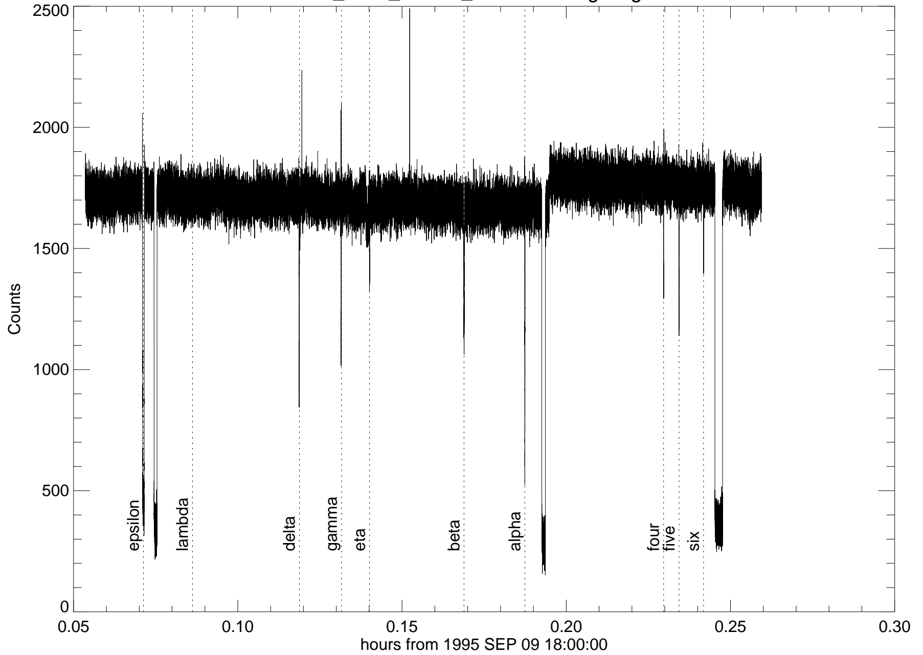
u134_saao_188cm_2220nm - rings ingress
