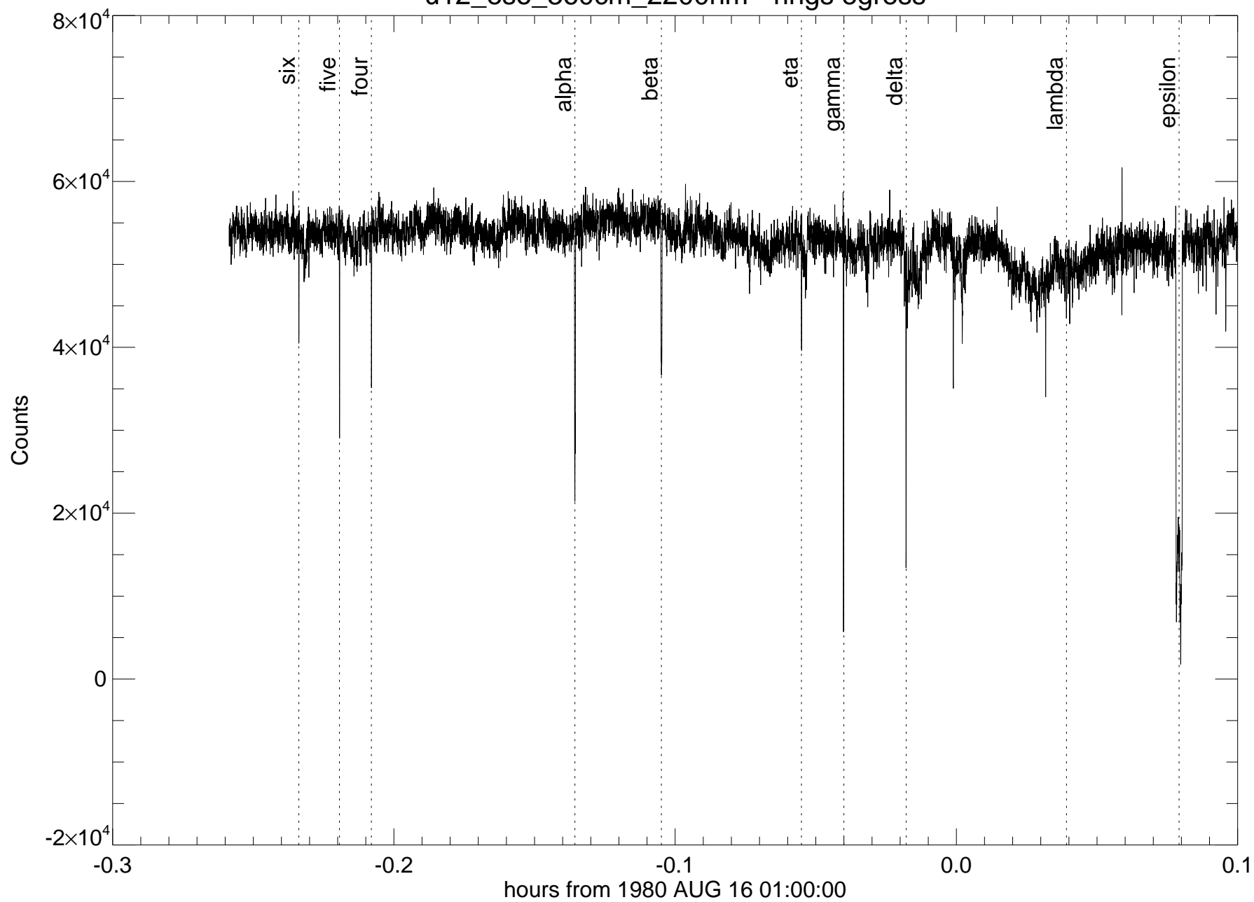
u12_eso_360cm_2200nm - rings egress
